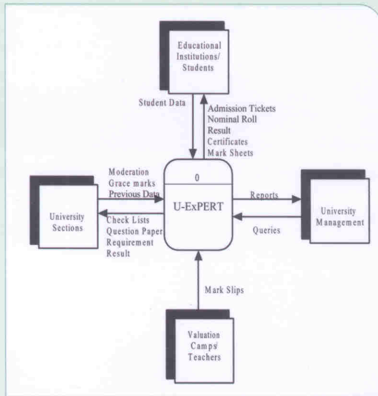
Context Diagrams for UExpert
